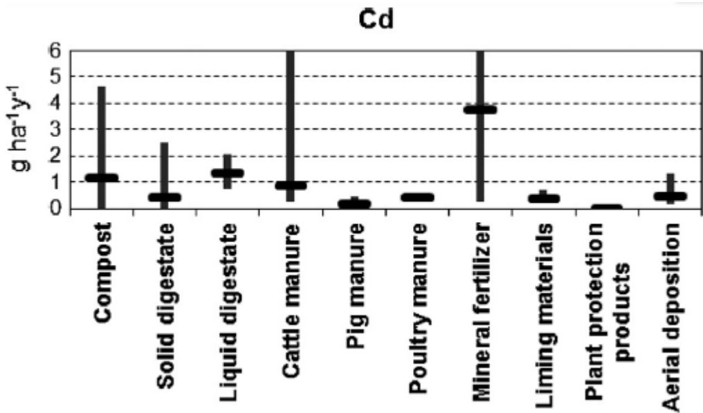
Figure 1: Estimated contributions of major inputs to soil cadmium load (Kupper et al 2014)
